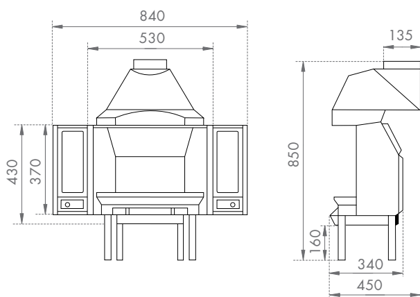
P54/55 | 1800 Multi-Fuel Fireplace†
