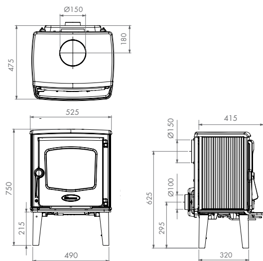
P18/19 | 525 Wood & Multi-Fuel Stoves
