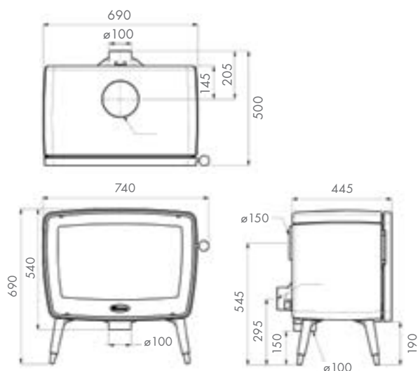
P34/35 | Vintage 50 Wood Stove
