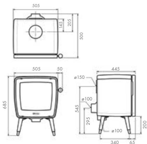
P34/35 | Vintage 50 Wood Stove
