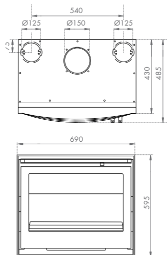
P52/53 | 2520 Cassette Fire
