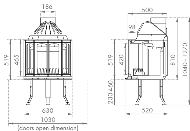
P60/61 | 2400CB Wood Fireplace†
