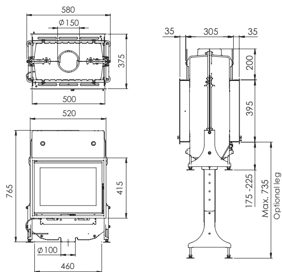
P50/51 | Zen 102 Double-Sided Cassette Fire†
