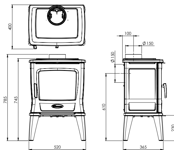
P20/21 | Tai 35 Wood Stove
