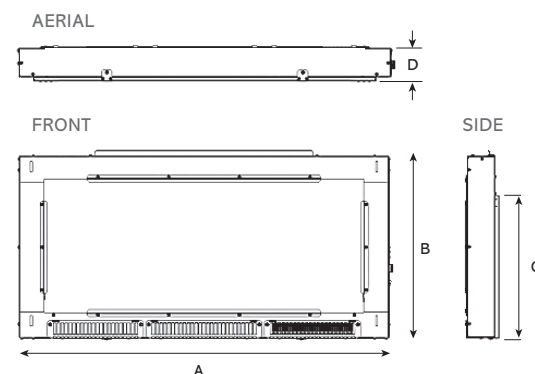
Studio Electric Fire Dimensions (mm)
