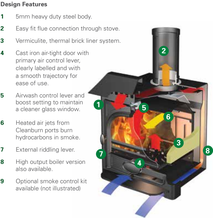
Stockton 7 Inset Convector with flat top, shown here in Matt Black burning logs.
